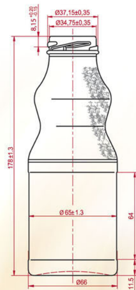
MIX 330 Filling capacity 330ml Brimful capacity 340 ± 7ml Weight - 275 gr Finish- "TO - 38"
