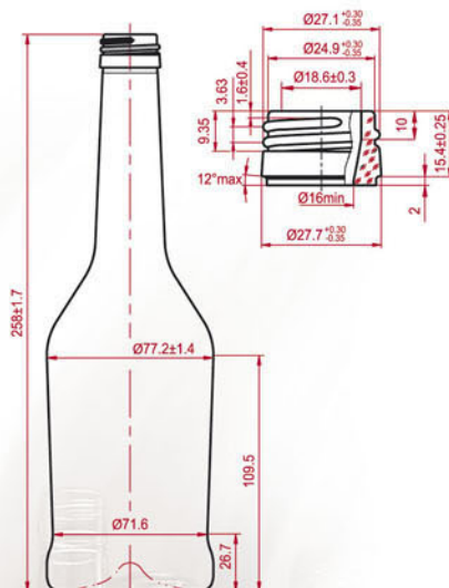
NAPOLEON 500 Filling capacity 500ml Brimful capacity 515 ± 10ml Weight - 385 gr Finish- "B-28-21" GOST 10117.2-2001
