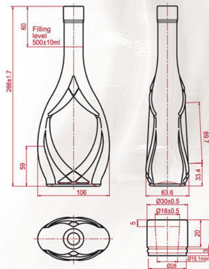
ICONA K 500 Filling capacity 500ml Weight - 420 gr Finish- "P-30-1"
