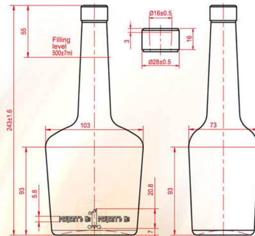
RETSEPT 500 Filling capacity 500 ml Brimful capacity 500 ± 7ml Weight - 415 gr Finish- "VP6"
