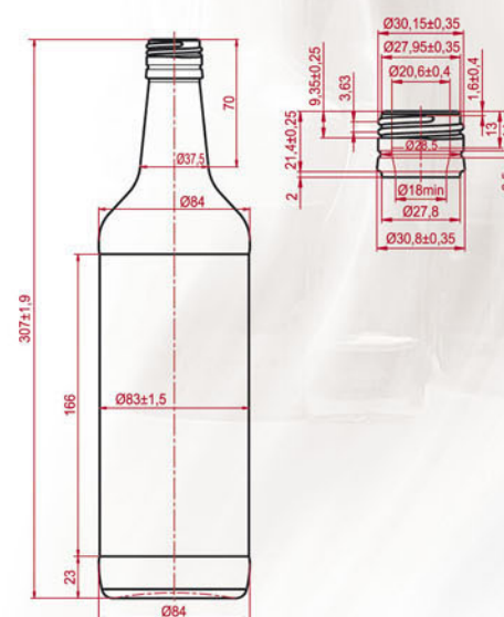
ANDREEVSKAYA 1000 Filling capacity 1000ml Brimful capacity 1030 ± 10ml Weight - 495 gr
