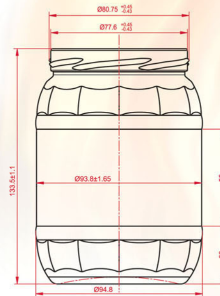
VIA 720 Brimful capacity 720 ± 15ml Weight - 298 gr Finish- "TO-82"
