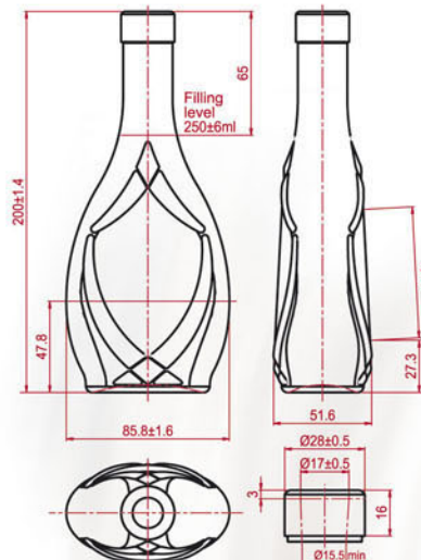
ICONA K 250 Filling capacity 250ml Weight - 255 gr Finish- "VP6- A"
