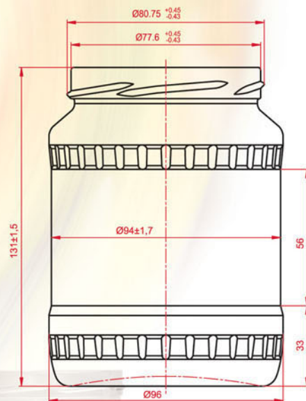
LIVIO 720 Brimful capacity 720 ± 15ml Weight - 295 gr Finish- "TO-82"
