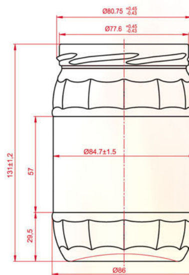
VIA 580 Brimful capacity 580 ± 10ml Weight - 257 gr Finish- "TO-82"
