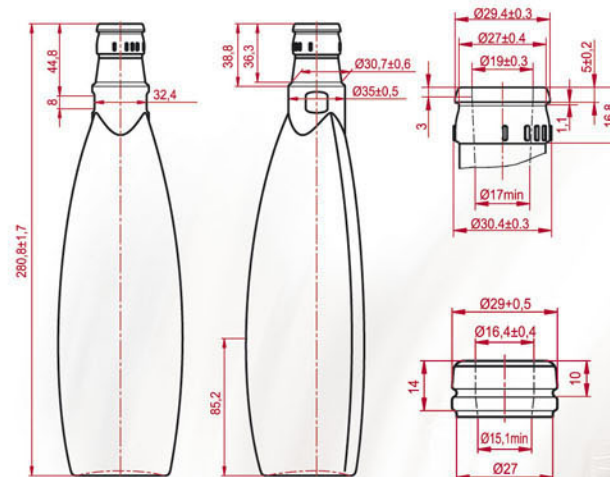
PARUS 500 Filling capacity 500ml Brimful capacity 520 ± 10ml Weight - 422 gr Finish- "КПМ-30-1" GOST 10117.2-2001 Finish- "VP2"
