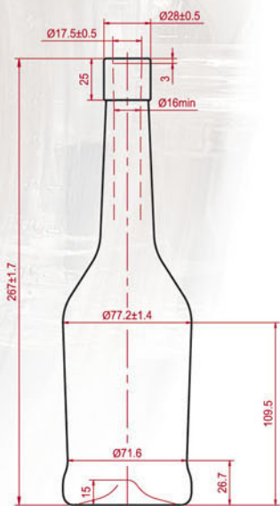
NAPOLEON 500 GH Filling capacity 500ml Brimful capacity 520 ± 10ml Weight - 395 gr Finish- "GH"
