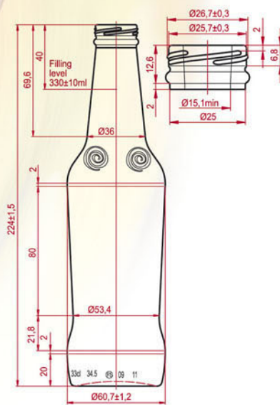
FESTIVAL 330 Filling capacity 330ml Weight - 200 gr Finish- "БКП-1"
