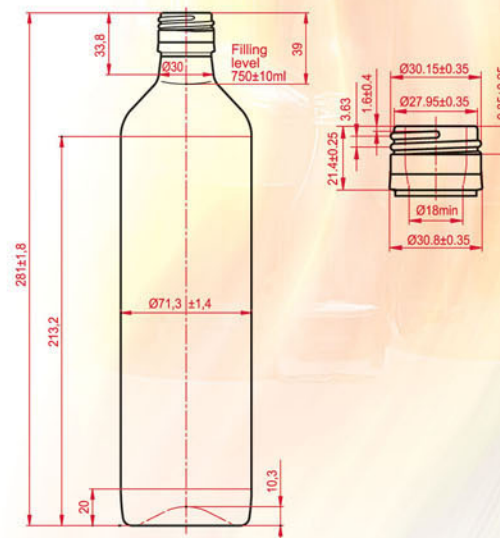
SPERONI 750 Filling capacity 750 ml Brimful capacity 750 ± 10ml Weight - 440 gr Finish- "B-31-3" GOST 10117.2-2001
