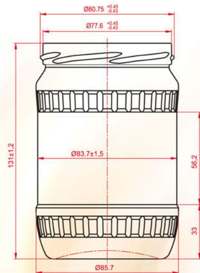
LIVIO 580 Brimful capacity 580 ± 10ml Weight - 255 gr Finish- "TO-82"
