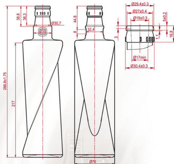
STALACTIT 500 Filling capacity 500ml Brimful capacity 520 ± 10ml Weight - 522 gr Finish- "КПМ-30-1" GOST 10117.2-2001
