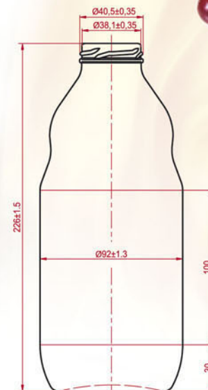
SOC 1000 Filling capacity 1000ml Brimful capacity 1040 ± 10ml Weight - 405 gr Finish- "TO - 43"
