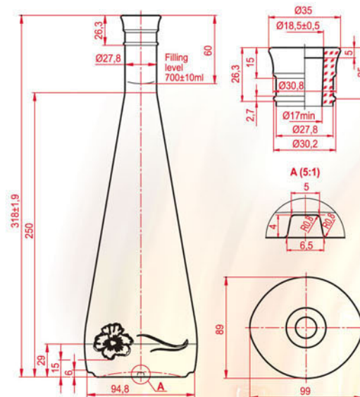
ANGELICA 700 Filling capacity 700 ml Brimful capacity 700 ± 10ml Weight - 550 gr Finish- "P-35-A"
