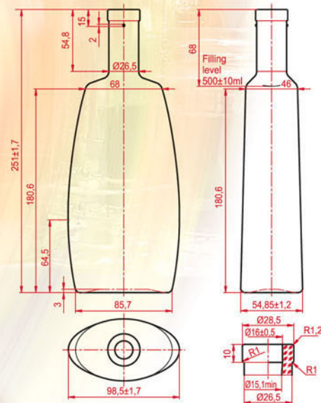
KOSA 500 Filling capacity 500 ml Brimful capacity 500 ± 10ml Weight - 425 gr Finish- "P-29"
